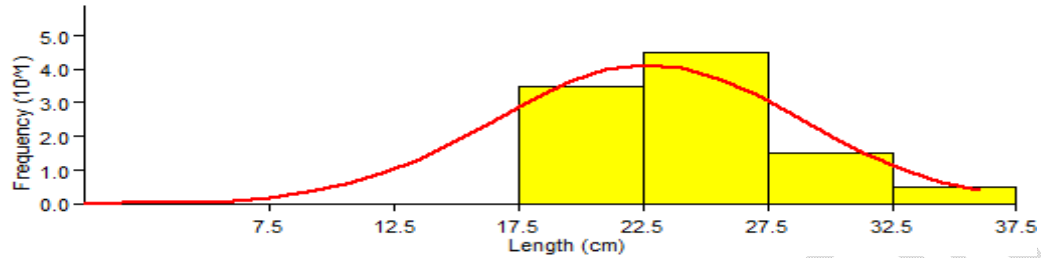
Fig (1). total length frequency distribution of S. schall from Upper Atbara and Setit complex dam.
